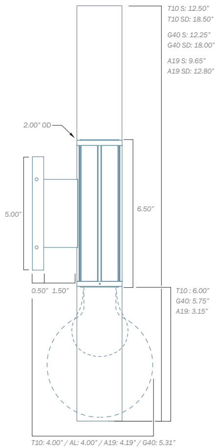
RPD14DS: Side view - seen here with two T10 bulbs (A19 and G40 in dashed lines).
