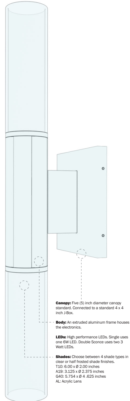
RPD14DS: Seen here with two clear T10 bulbs with a black finish.
